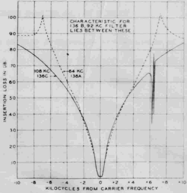
Fig. 10 - Schematic and Typical Insertion Loss Characteristics of the Channel Carrier Supply Filters -
